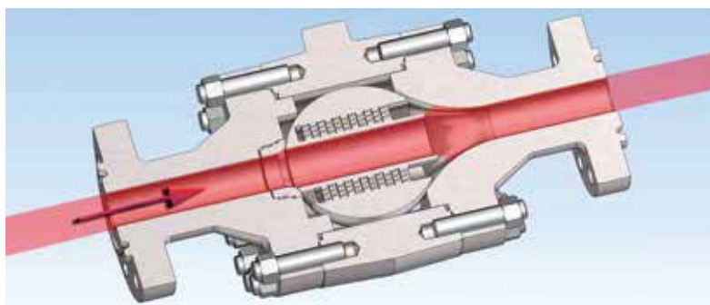
FULLY OPEN Zero pressure drop
