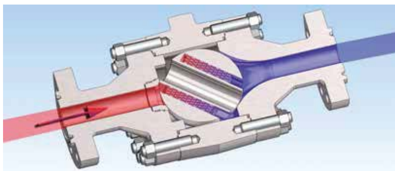
THROTTLING POSITION High pressure drop
